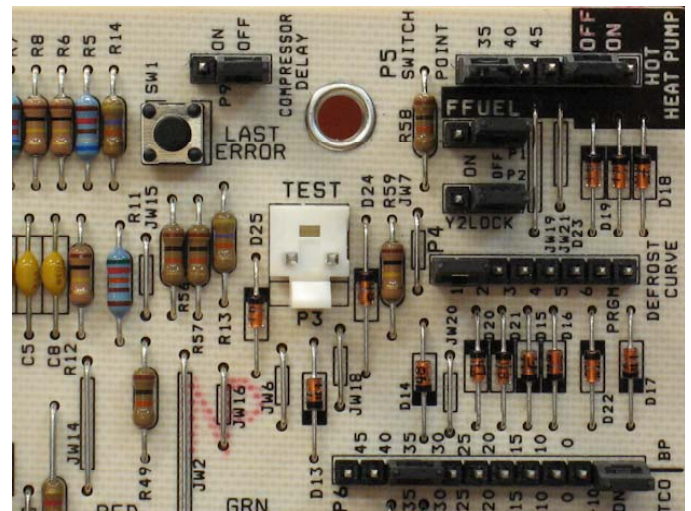
FIGURE 2: Jumper Inputs
